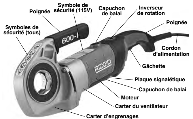
Figure 1 – Fileteuse 600-I
