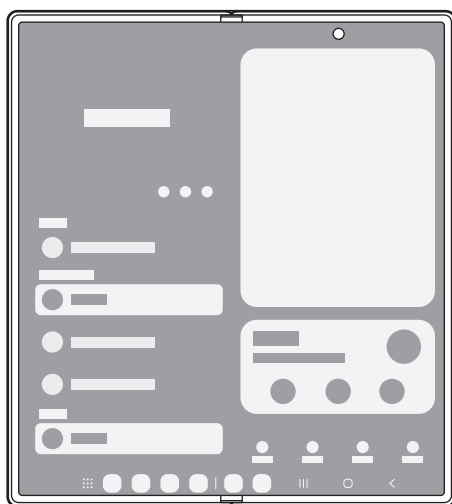
Main screen
