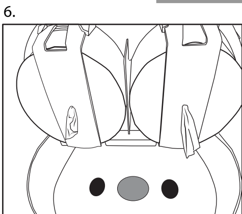
With the inner doors closed, pull 2 -3 sheets of from each roll to ensure no paper jams
