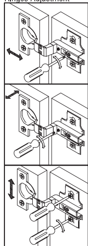
Hinges Adjustment
